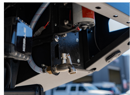
12V Water Pump Included with 70L Under-Tray Water Tank
